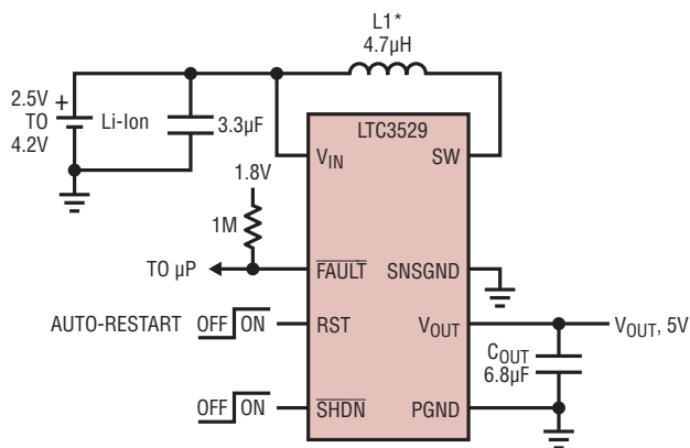
Li-Ion Battery to 5V at 100mA or 500mA for USB OTG Host Supply
