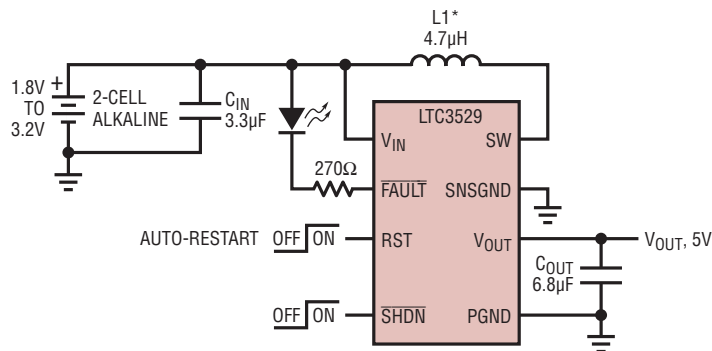
2 Alkaline Cells to 5V at 350mA
