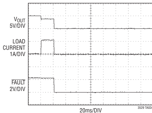
Overcurrent Event V RST Low
